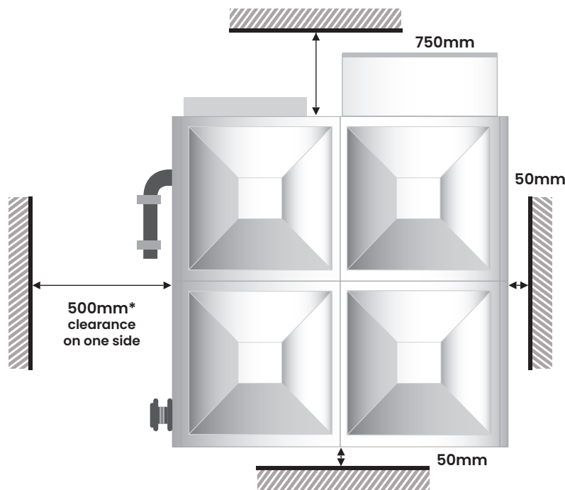
Plan view of tank with clearance measurements
